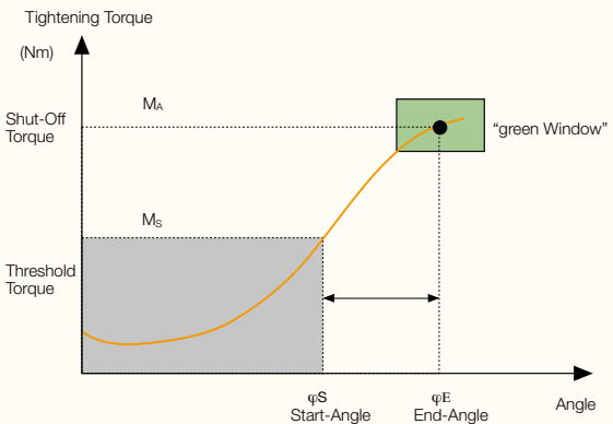
Additional angle monitoring at torque-controlled tightening
