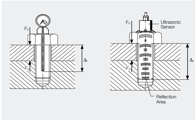
Length measurement
