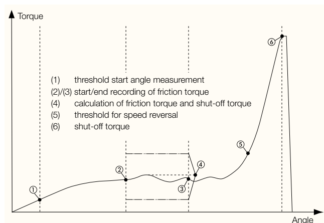
Angle-controlled tightening
